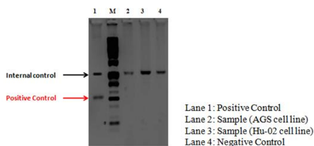
Figure 1. mycoplasma quality control test using the PCR method
