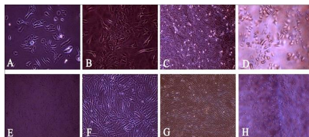
Figure 2. evaluating mycoplasmatic infection in cell lines using DNA painting (Hoechst method)
